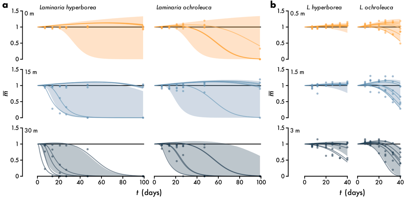
Fig. 5. Example 4: the effect of light attenuation with depth on the decomposition of Laminaria hyperborea and Laminaria ochroleuca ex situ (a, n = 210 , data from Frontier et al. 2021 ) and in situ (b, n = 252 , data from Frontier et al. 2022 ), shown as normalised remaining mass over time t . Data are plotted alongside predictions of the mean \bar{m} where lines are medians per replicate and intervals are the central 90% of posterior probability across replicates (Eq. 19, cf. Fig. S5 ).
