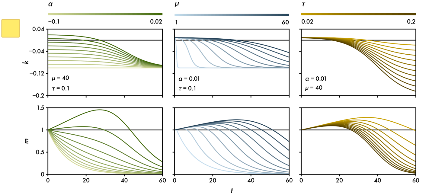
Fig. 1. The mathematical model: the effect of varying \alpha , \mu and \tau on the trajectory of the exponential rate k (Eq. 6) and normalised remaining mass m (Eq. 9) over time t (cf. Fig. S1).
