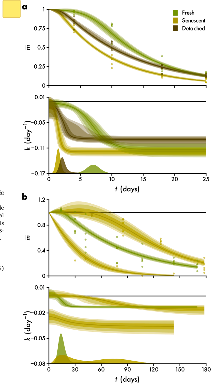
Fig. 3. Example 2: the effect of senescence on the decomposition of Macrocystis pyrifera (a, n = 61 , data from Hamersley et al. 2015) and Laminaria hyperborea (b, n = 63 , data from de Bettignies et al. 2020), shown as normalised remaining mass over time t . Data are plotted alongside predictions of the mean \bar{m} , the time-variant exponential rate k and photosynthetic half-life \mu (Eqs. 16 and 17, cf. Fig. S3). Lines and intervals are medians and the central 50, 80 and 90% of posterior probability. Distributions are kernel density estimates of the probability density function of \mu .
