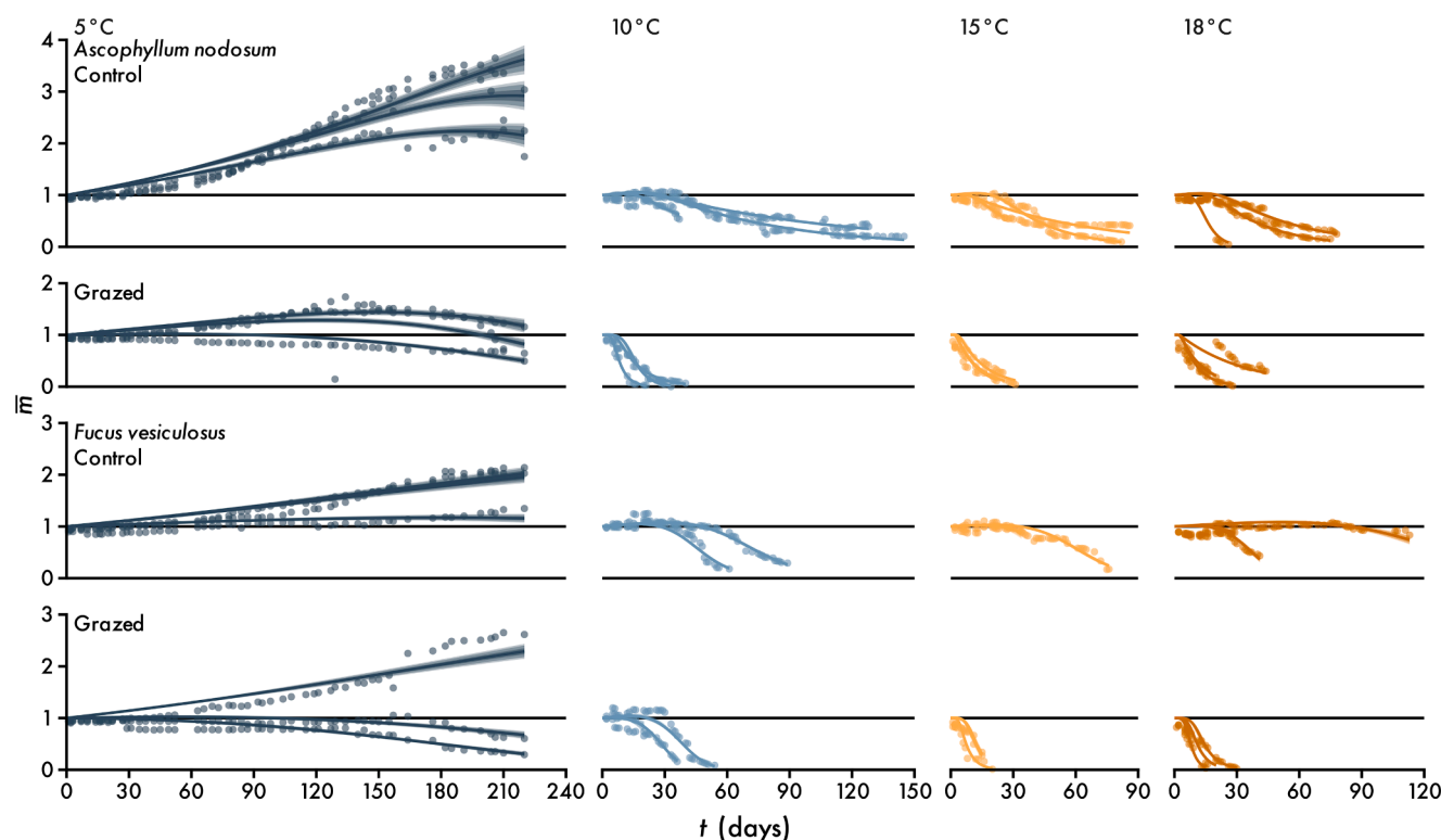
Fig. 6. Example 5: the effect of temperature and grazing on the decomposition of floating Ascophyllum nodosum and Fucus vesiculosus ( n = 1651 , data from Vandendriessche et al. 2007), shown as normalised remaining mass over time t . Data are plotted alongside predictions of the mean \bar{m} for each replicate (Eq. 20, cf. Fig. S6). Lines and intervals are medians and the central 50, 80 and 90% of posterior probability.
